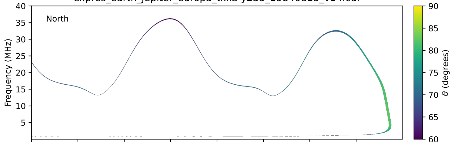
expres_earth_jupiter_europa_txka-y235_19840813_v14.cdf
