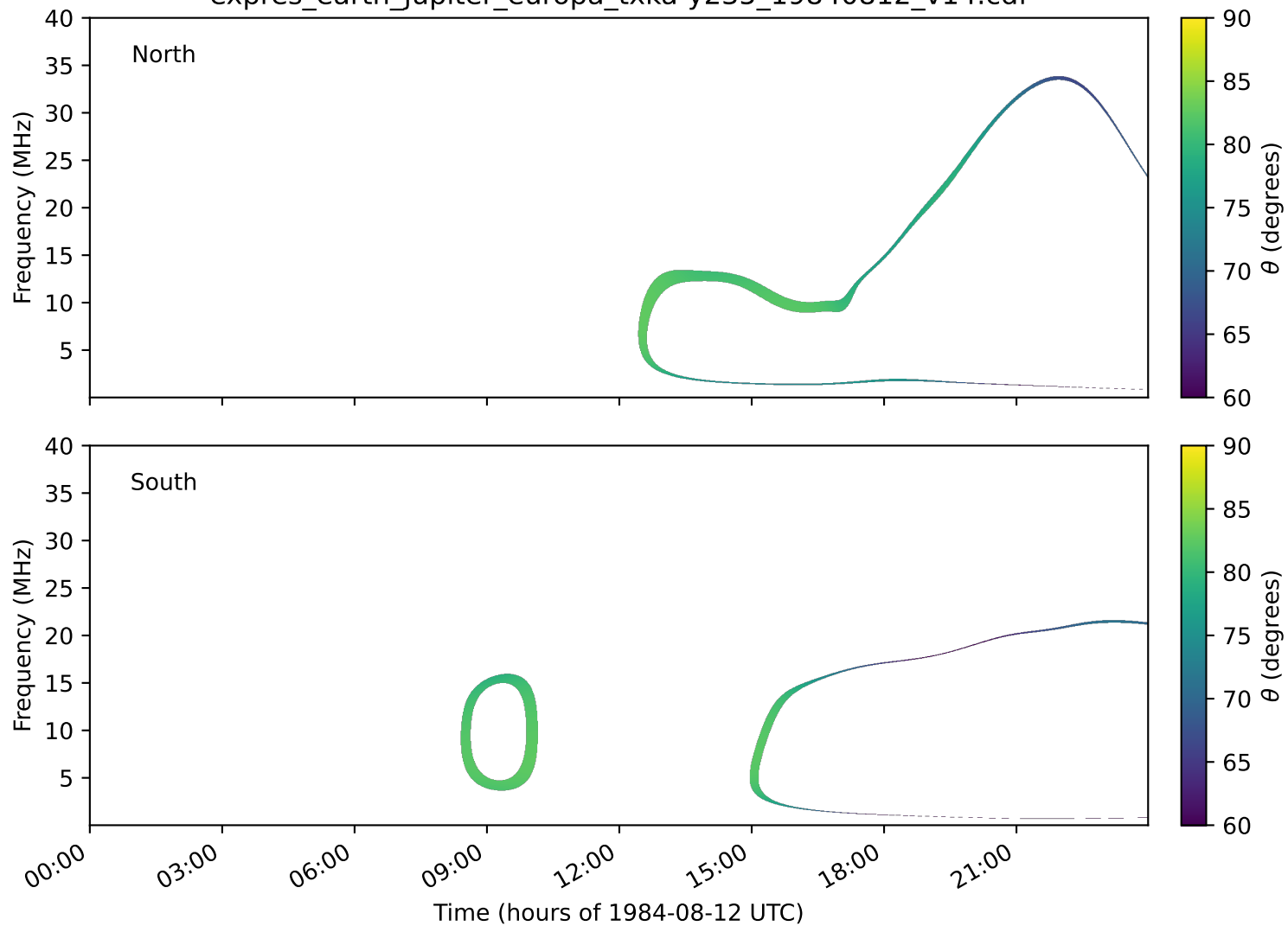
expres_earth_jupiter_europa_txka-y235_19840812_v14.cdf
