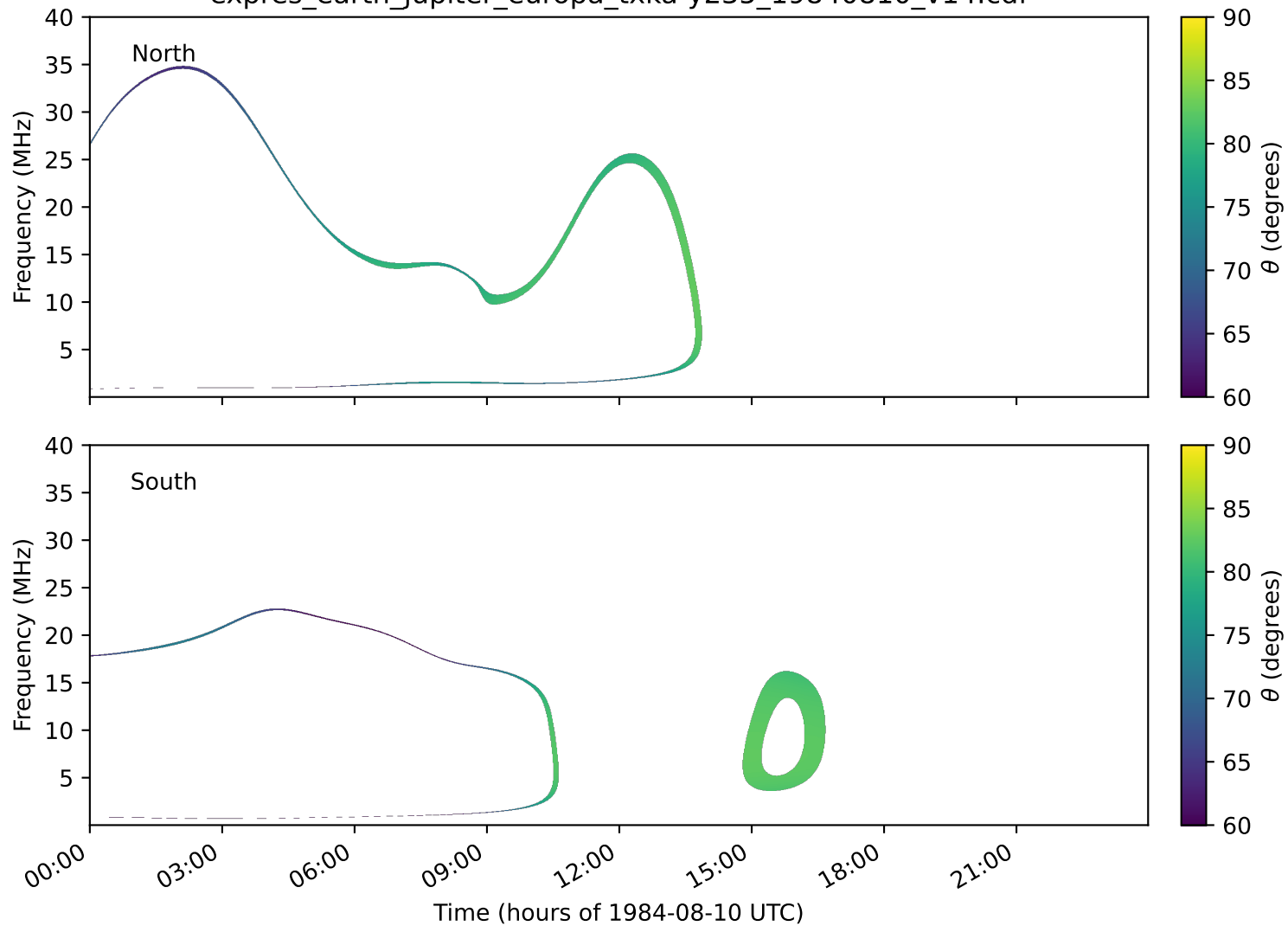
expres_earth_jupiter_europa_txka-y235_19840810_v14.cdf
