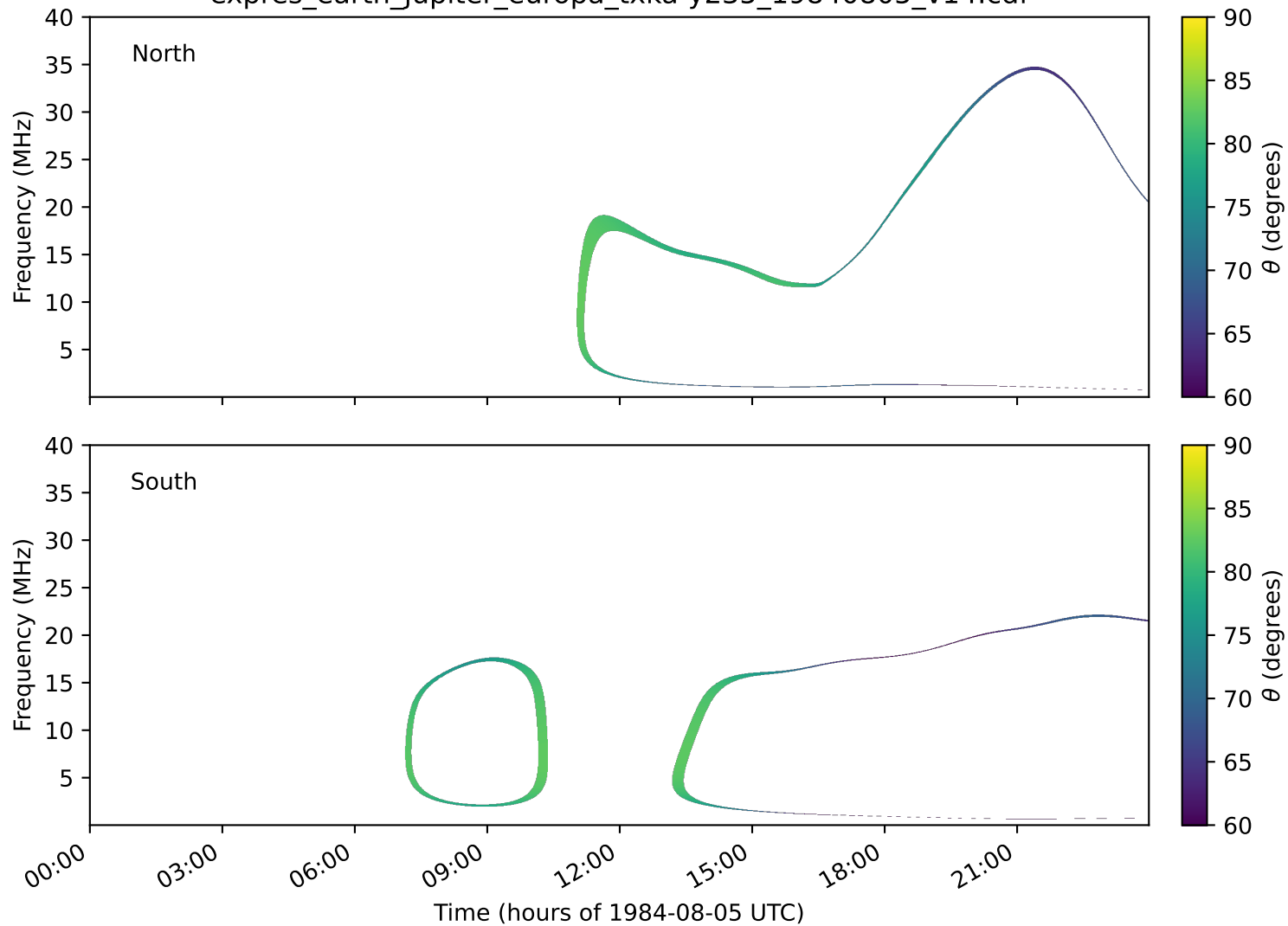
expres_earth_jupiter_europa_txka-y235_19840805_v14.cdf
