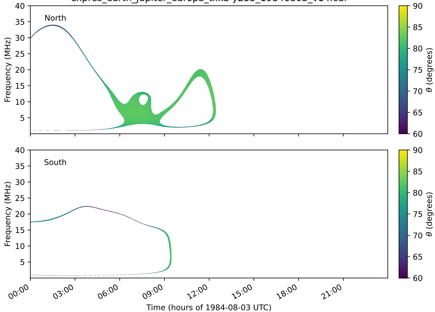
expres_earth_jupiter_europa_txka-y235_19840803_v14.cdf
