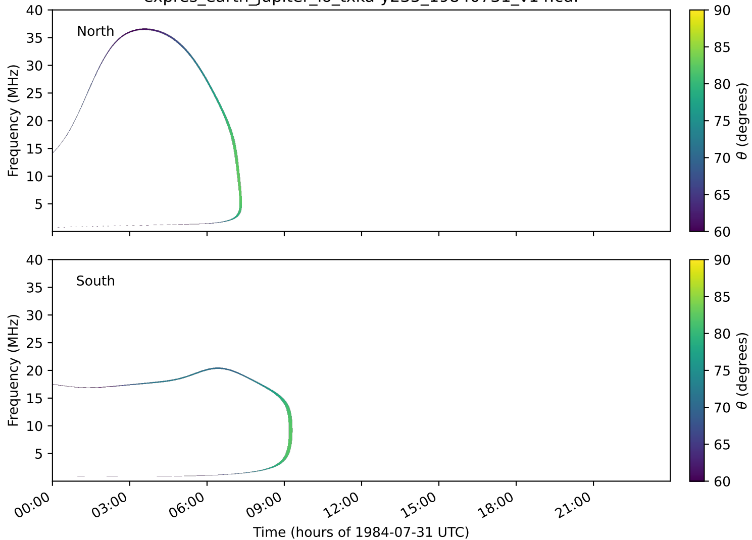
expres_earth_jupiter_io_txka-y235_19840731_v14.cdf
