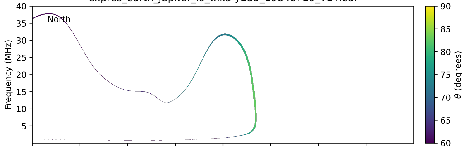
expres_earth_jupiter_io_txka-y235_19840729_v14.cdf
