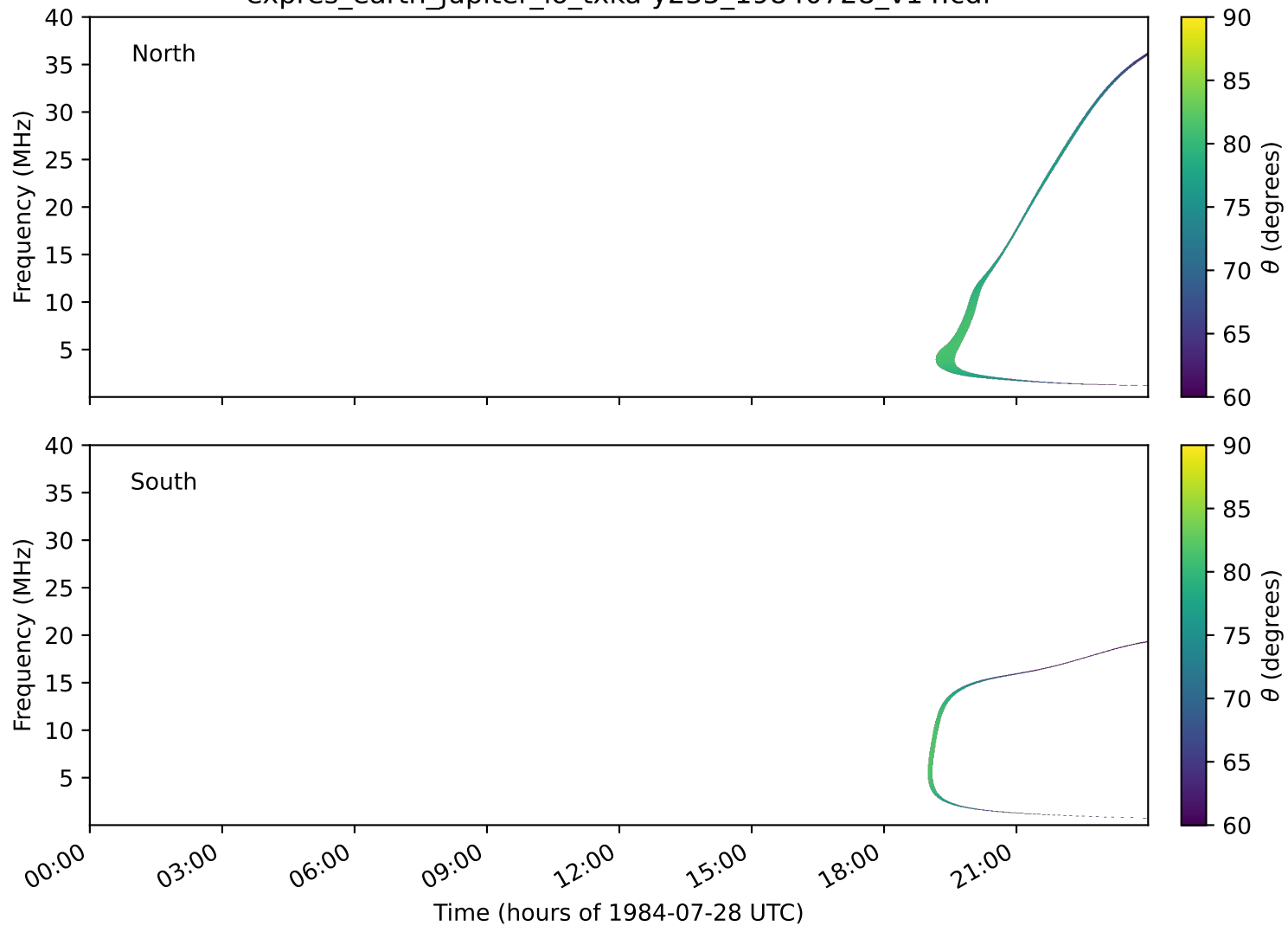
expres_earth_jupiter_io_txka-y235_19840728_v14.cdf
