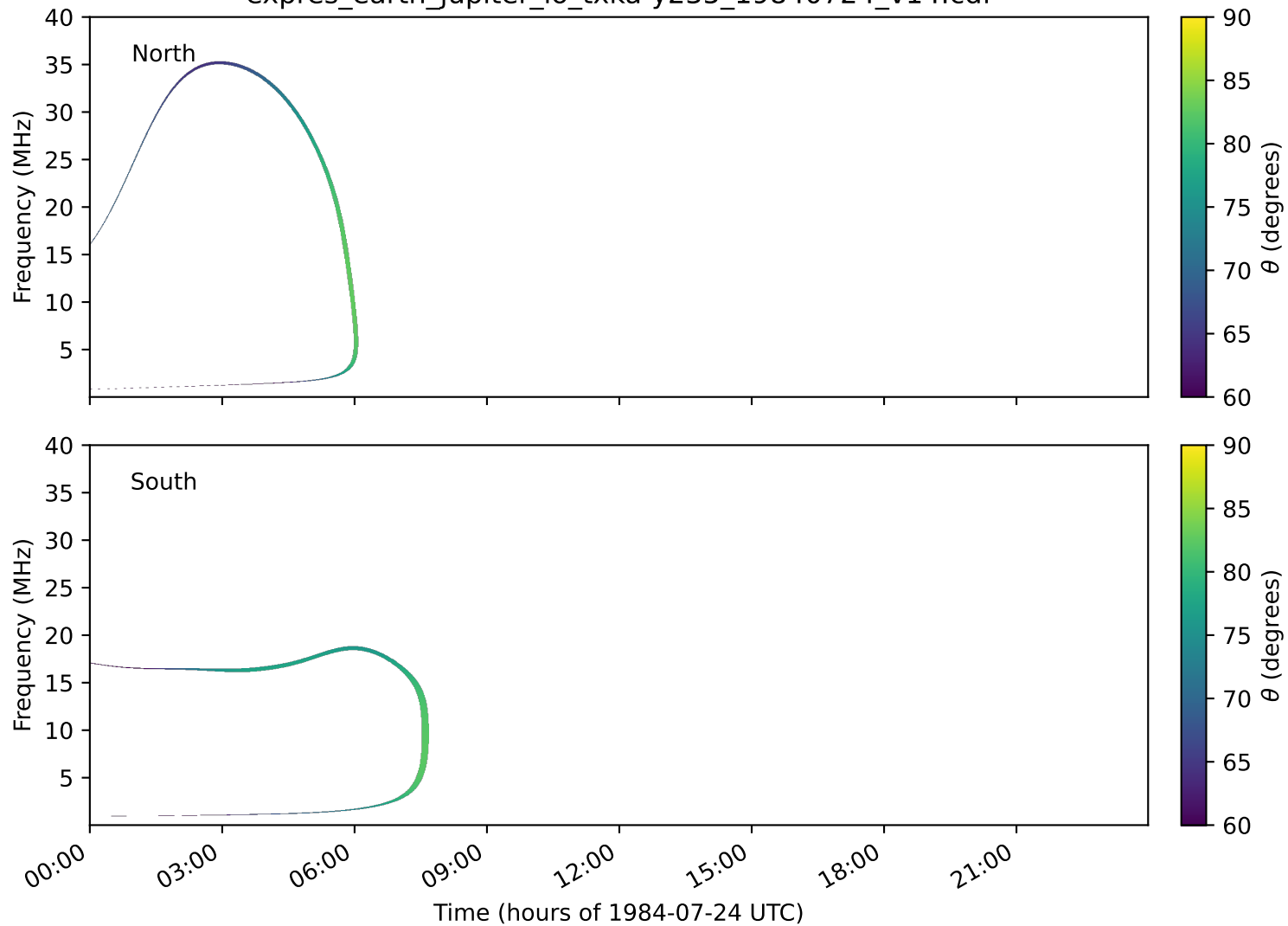
expres_earth_jupiter_io_txka-y235_19840724_v14.cdf
