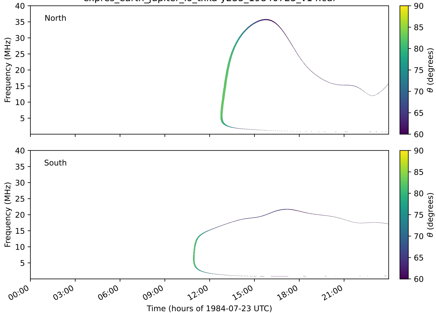
expres_earth_jupiter_io_txka-y235_19840723_v14.cdf
