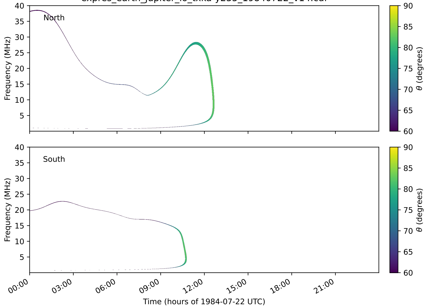
expres_earth_jupiter_io_txka-y235_19840722_v14.cdf
