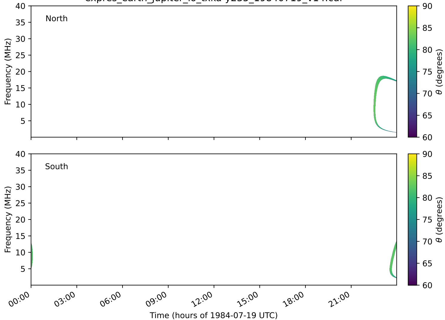
expres_earth_jupiter_io_txka-y235_19840719_v14.cdf
