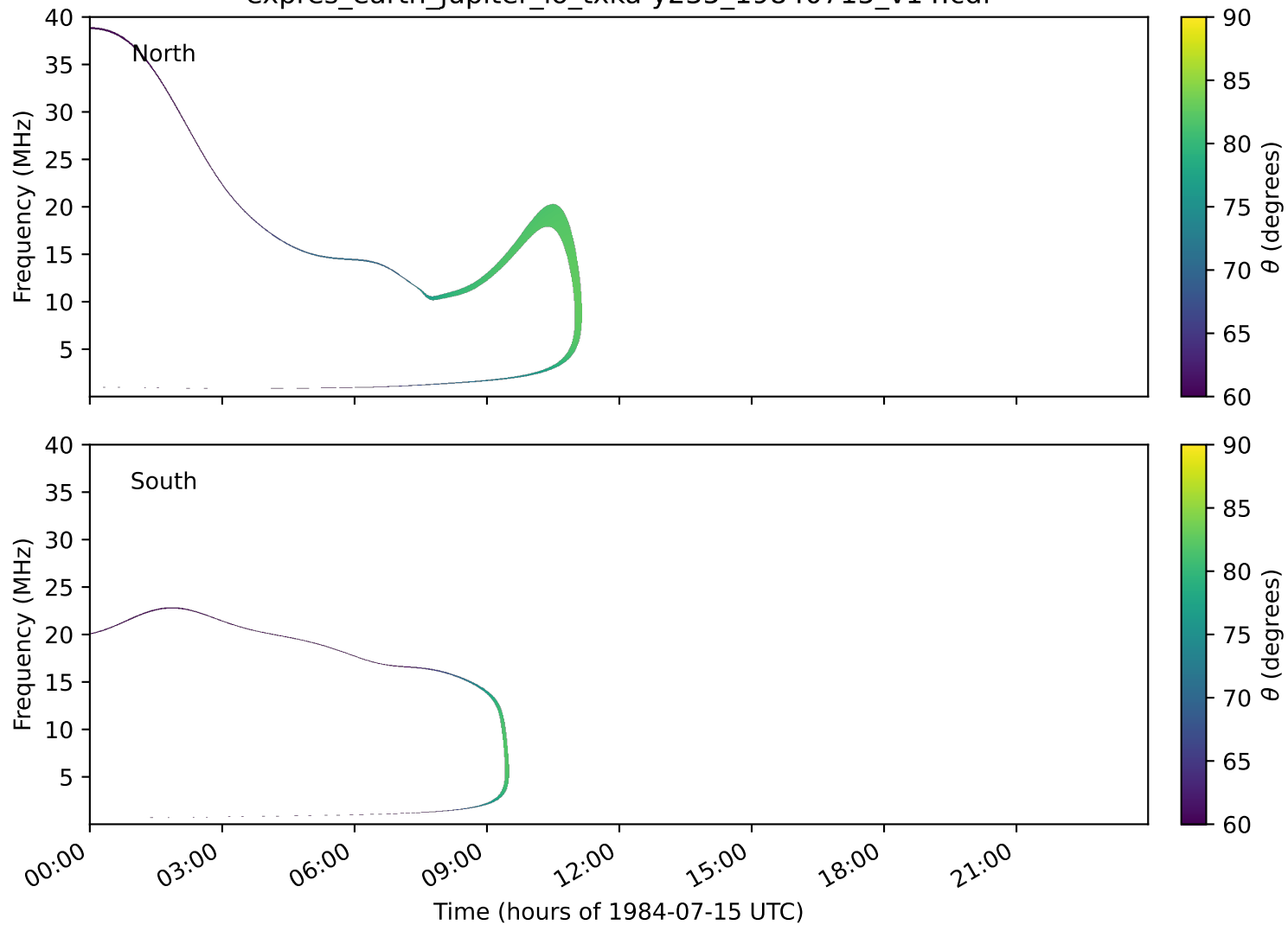
expres_earth_jupiter_io_txka-y235_19840715_v14.cdf
