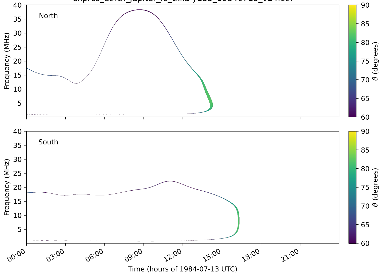
expres_earth_jupiter_io_txka-y235_19840713_v14.cdf
