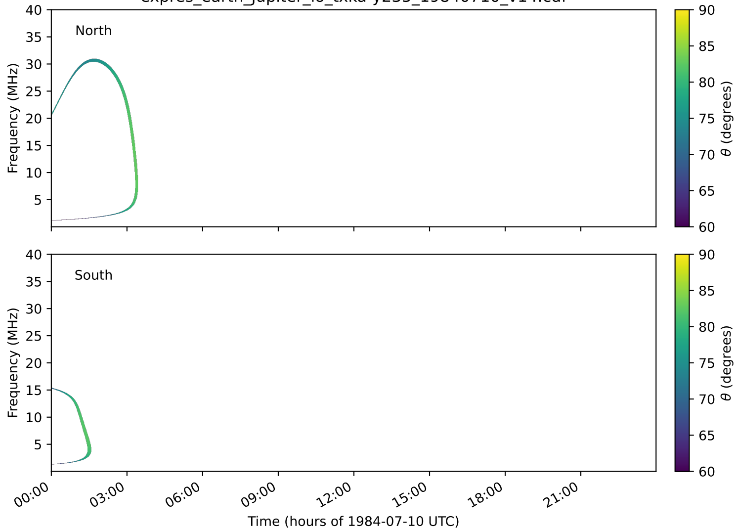
expres_earth_jupiter_io_txka-y235_19840710_v14.cdf
