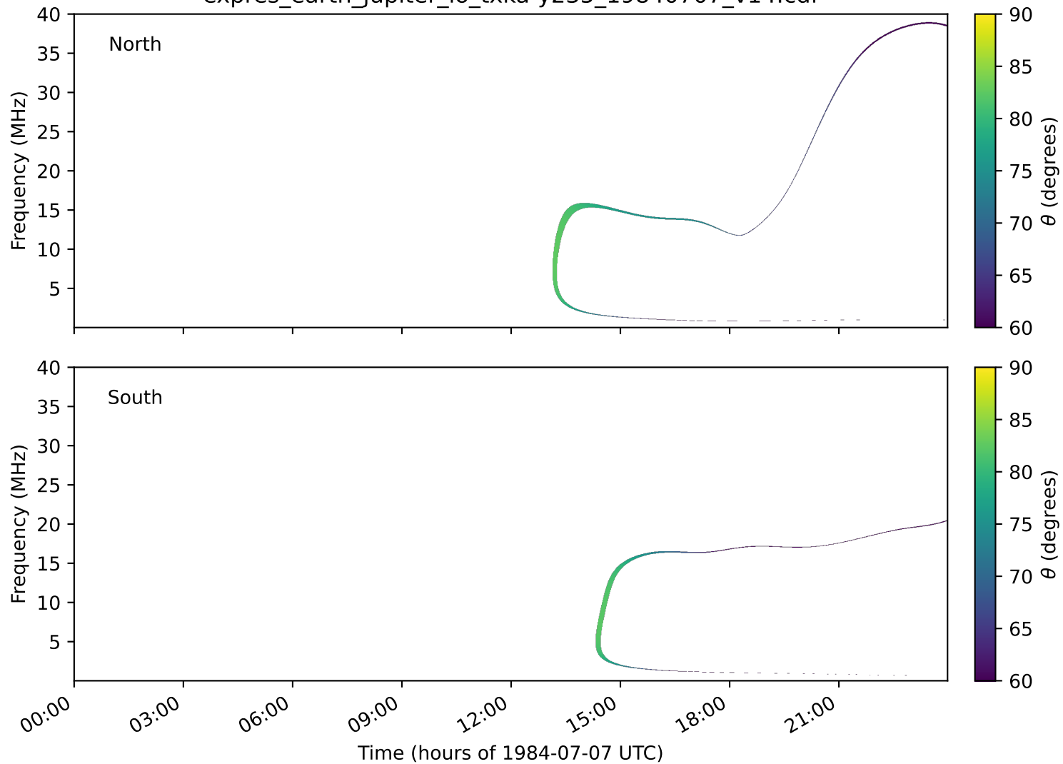
expres_earth_jupiter_io_txka-y235_19840707_v14.cdf
