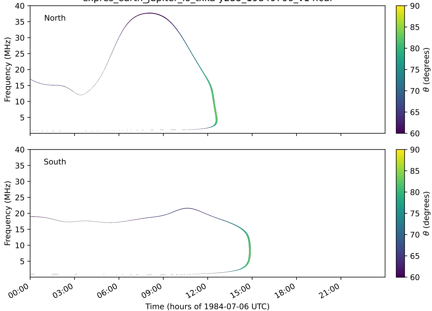
expres_earth_jupiter_io_txka-y235_19840706_v14.cdf
