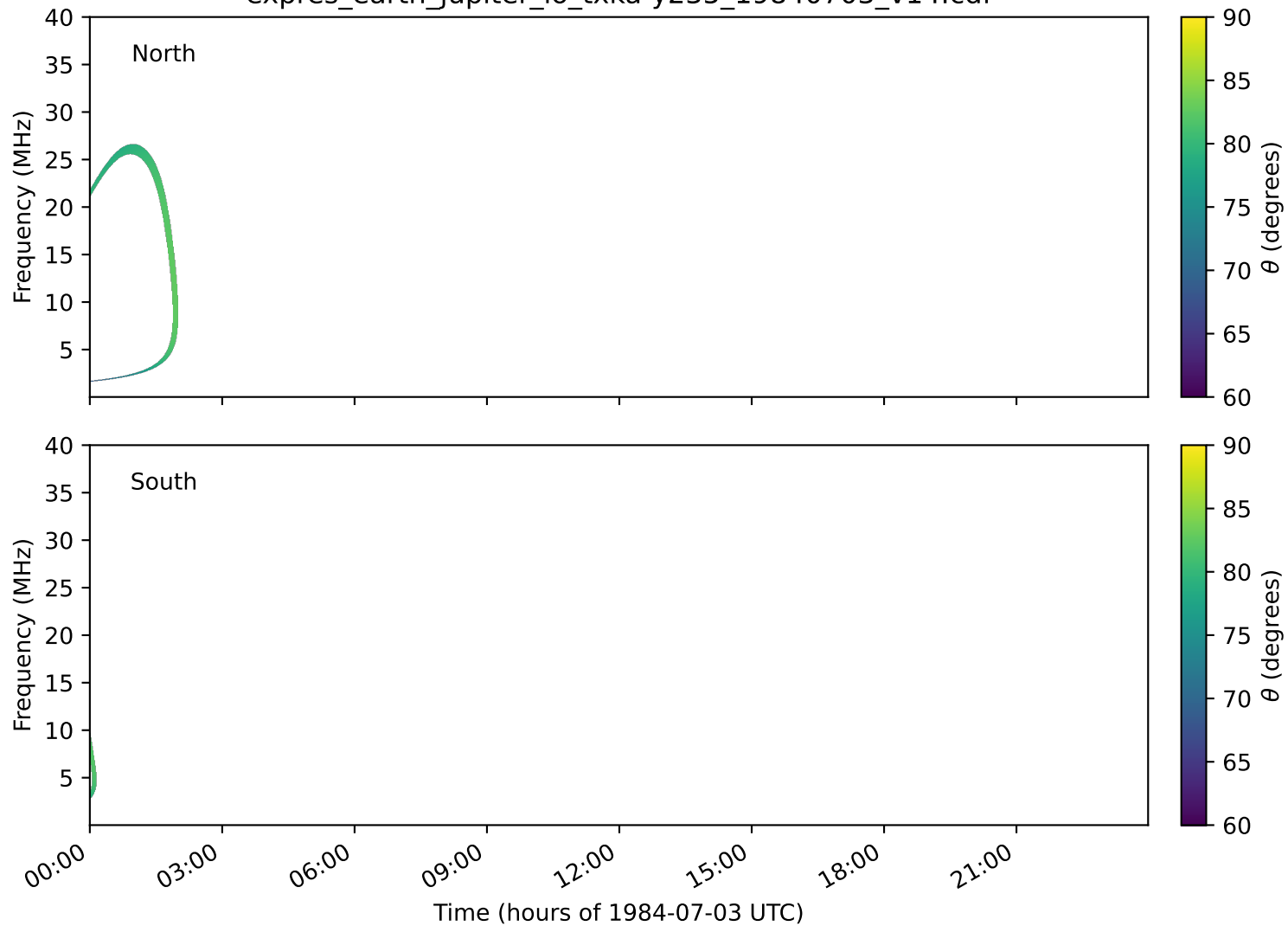
expres_earth_jupiter_io_txka-y235_19840703_v14.cdf
