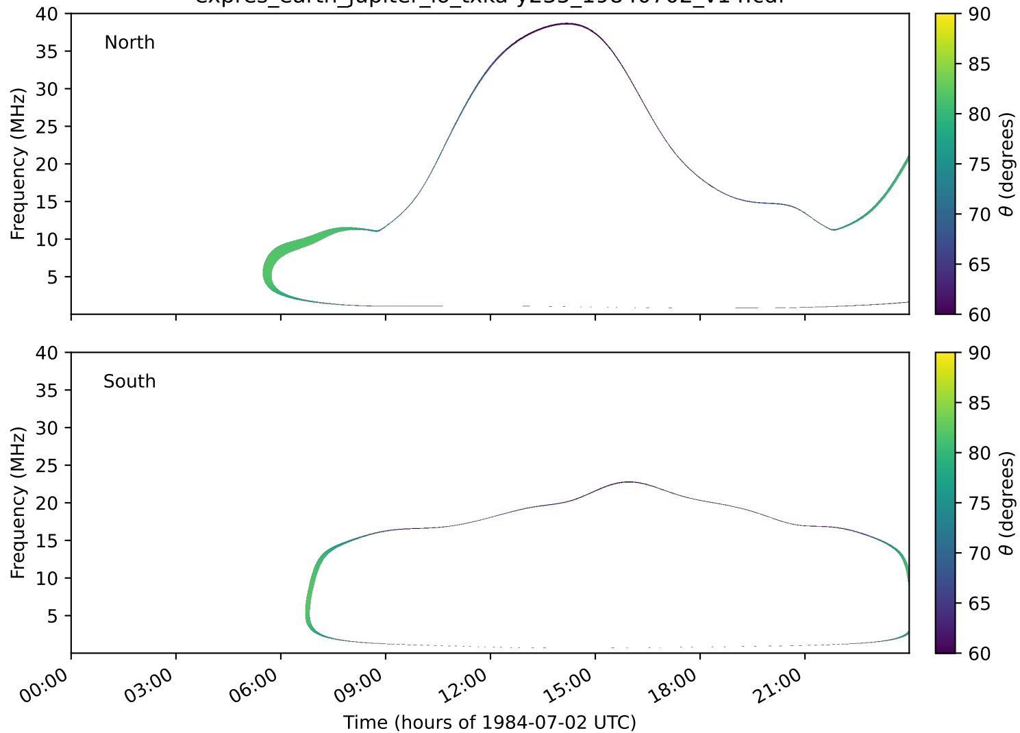
expres_earth_jupiter_io_txka-y235_19840702_v14.cdf
