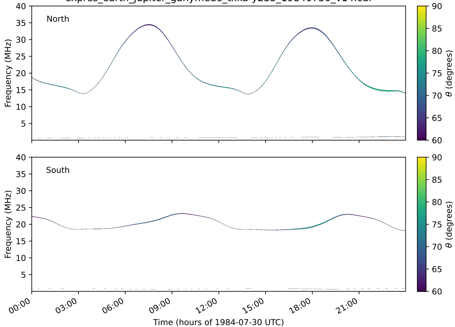
expres_earth_jupiter_ganymede_txka-y235_19840730_v14.cdf
