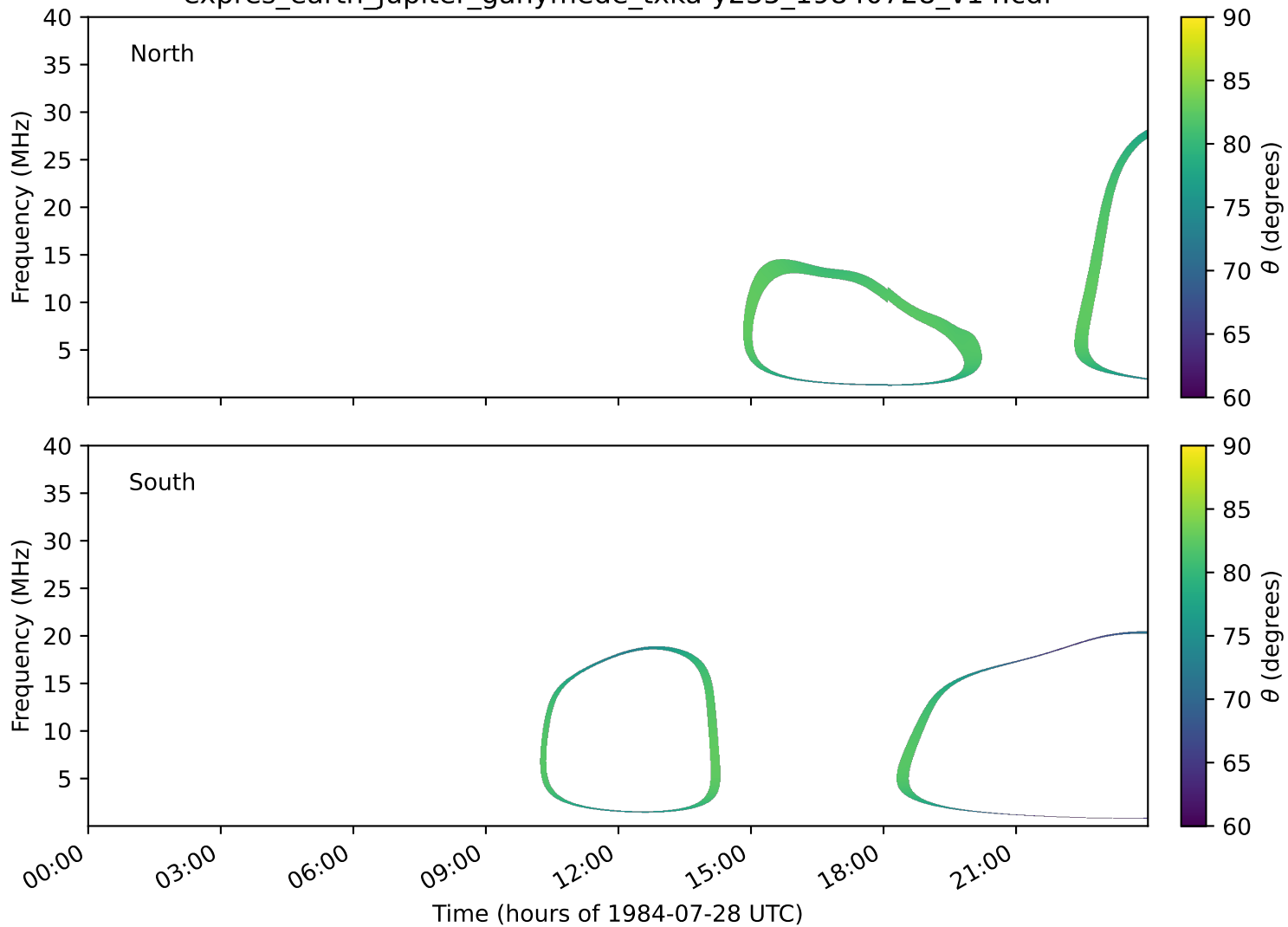
expres_earth_jupiter_ganymede_txka-y235_19840728_v14.cdf
