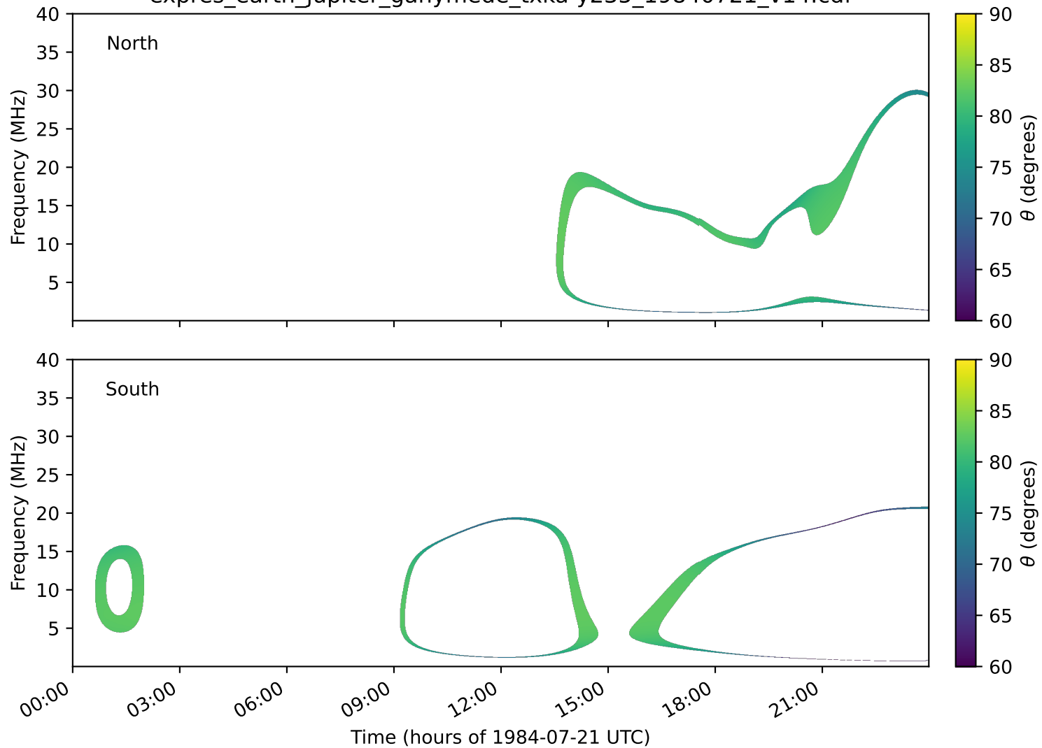
expres_earth_jupiter_ganymede_txka-y235_19840721_v14.cdf
