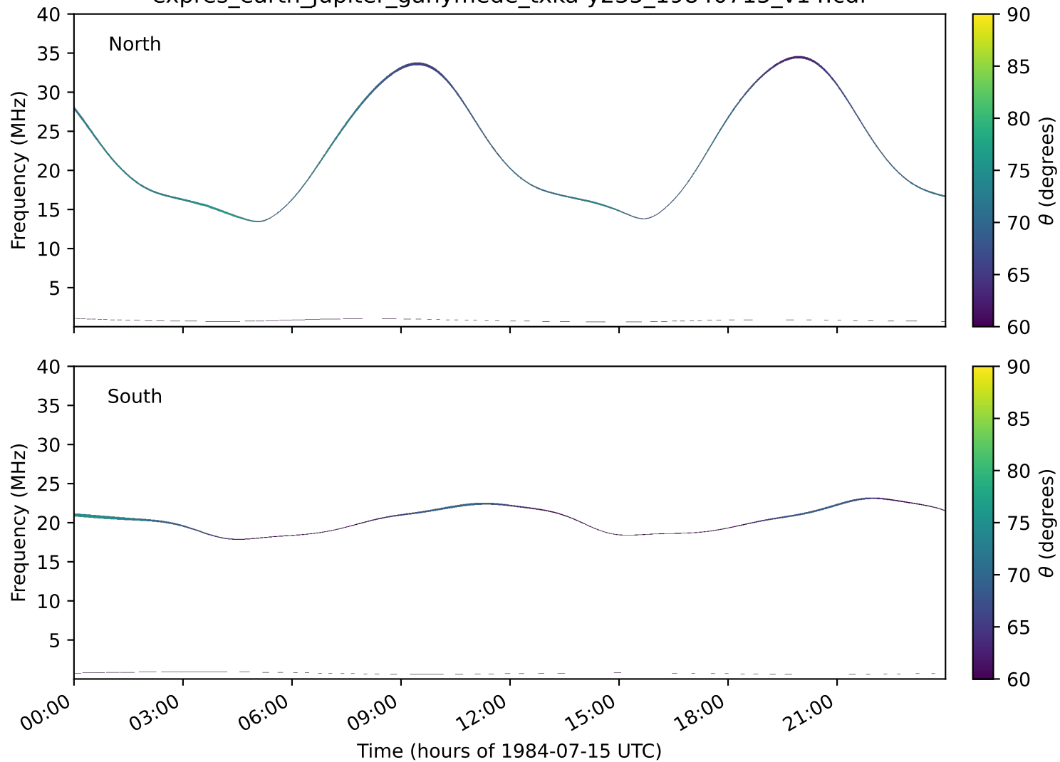
expres_earth_jupiter_ganymede_txka-y235_19840715_v14.cdf
