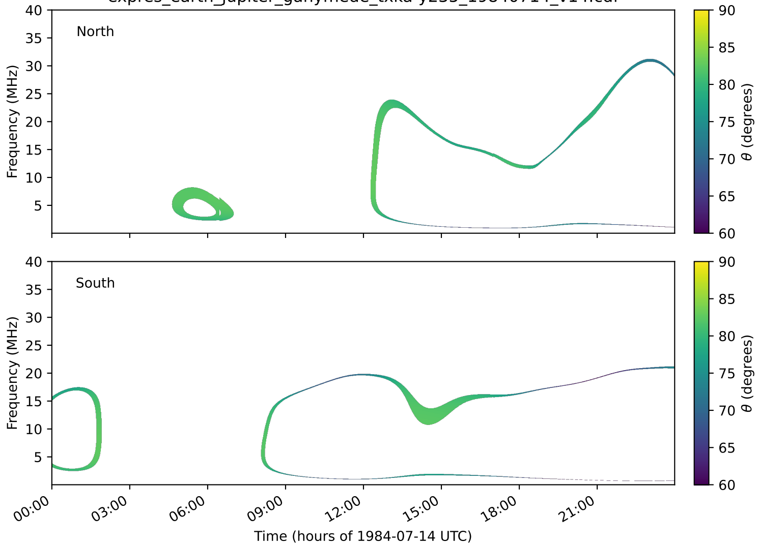
expres_earth_jupiter_ganymede_txka-y235_19840714_v14.cdf
