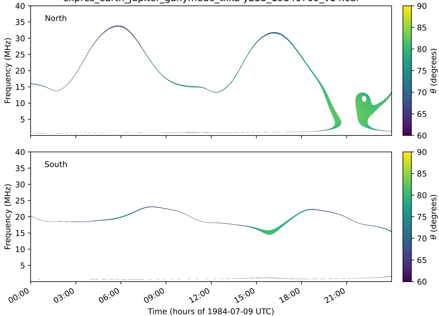
expres_earth_jupiter_ganymede_txka-y235_19840709_v14.cdf
