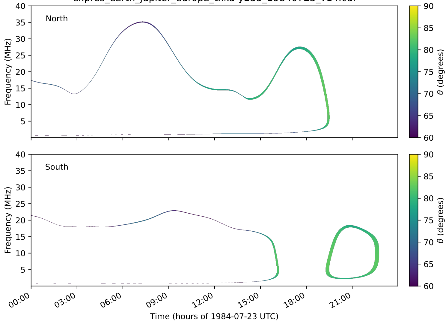
expres_earth_jupiter_europa_txka-y235_19840723_v14.cdf
