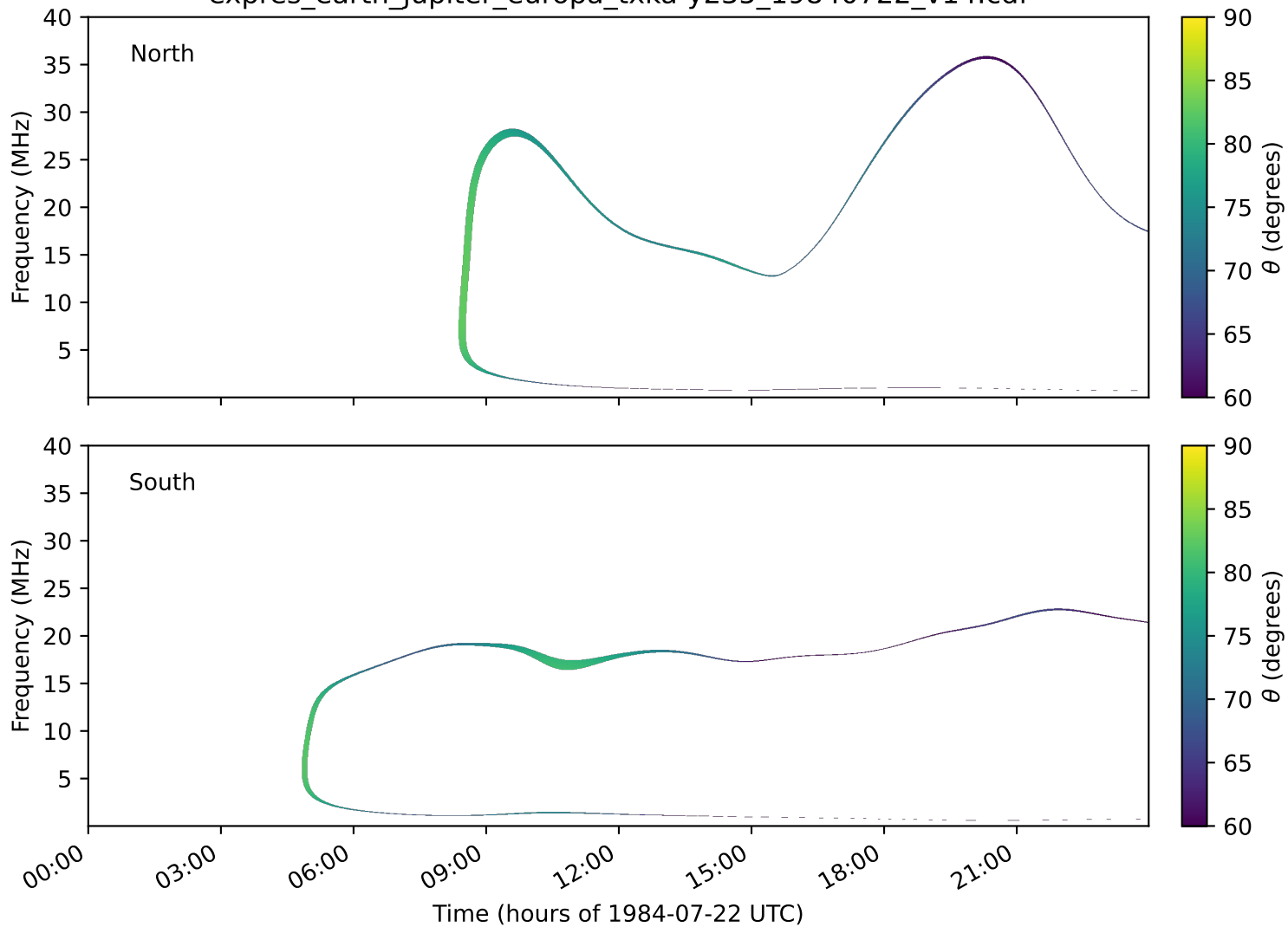
expres_earth_jupiter_europa_txka-y235_19840722_v14.cdf
