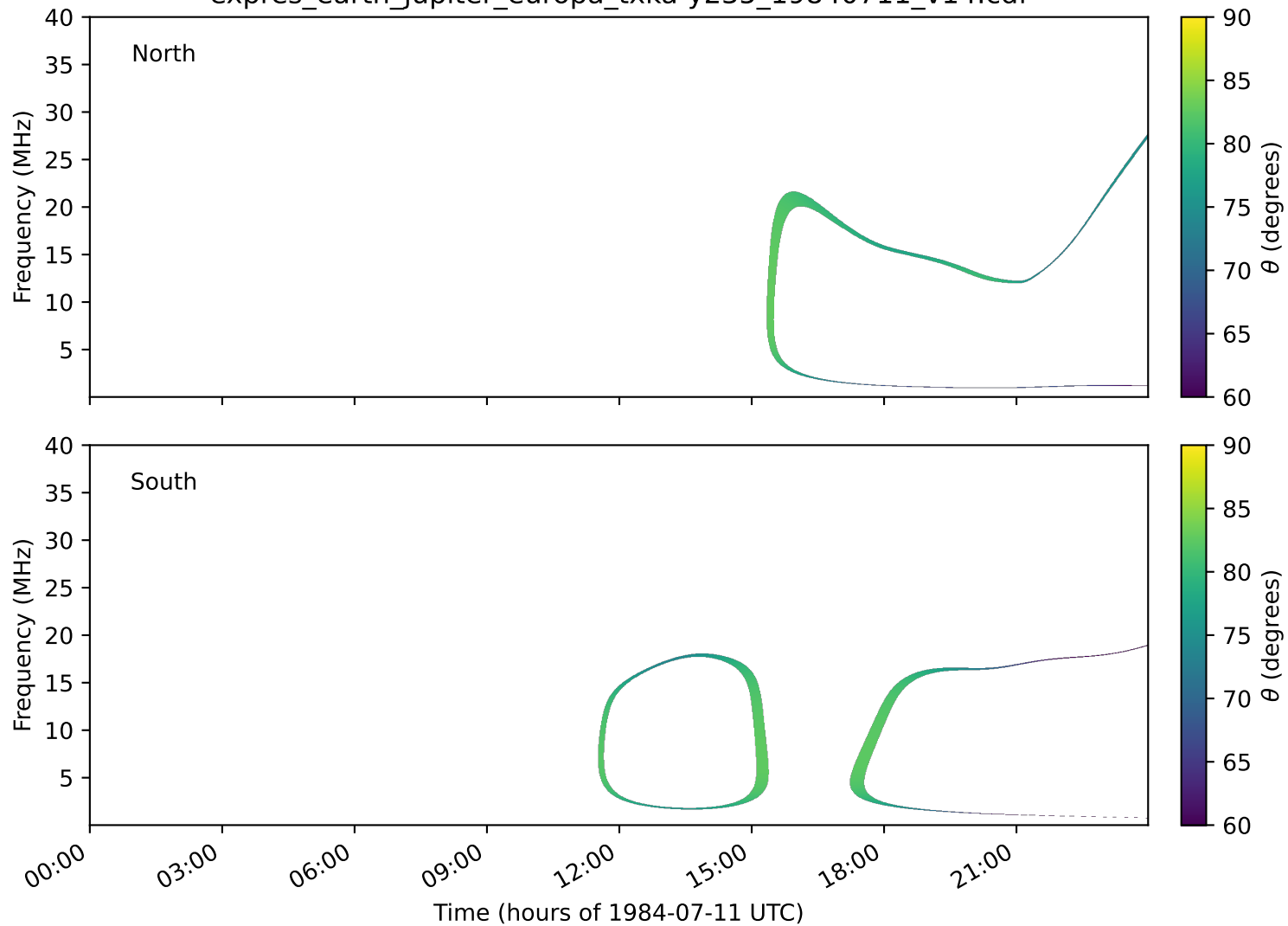
expres_earth_jupiter_europa_txka-y235_19840711_v14.cdf
