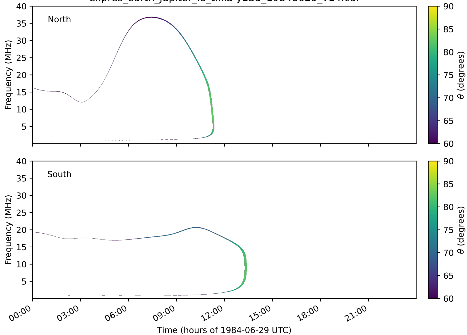
expres_earth_jupiter_io_txka-y235_19840629_v14.cdf
