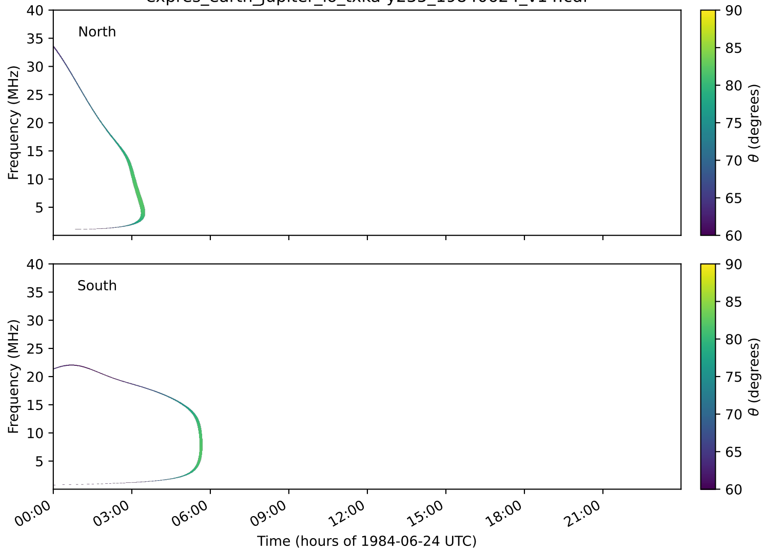
expres_earth_jupiter_io_txka-y235_19840624_v14.cdf
