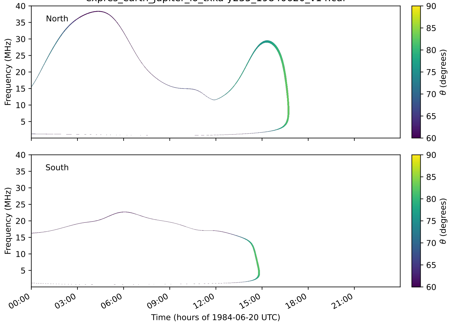
expres_earth_jupiter_io_txka-y235_19840620_v14.cdf
