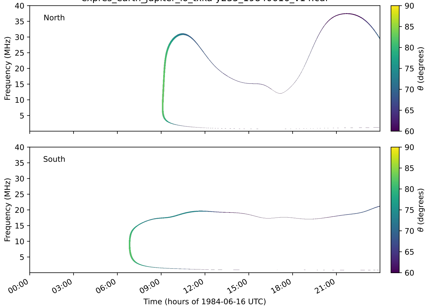
expres_earth_jupiter_io_txka-y235_19840616_v14.cdf
