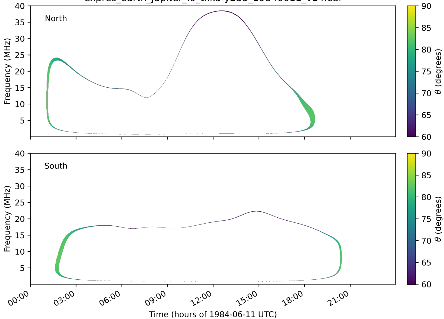
expres_earth_jupiter_io_txka-y235_19840611_v14.cdf
