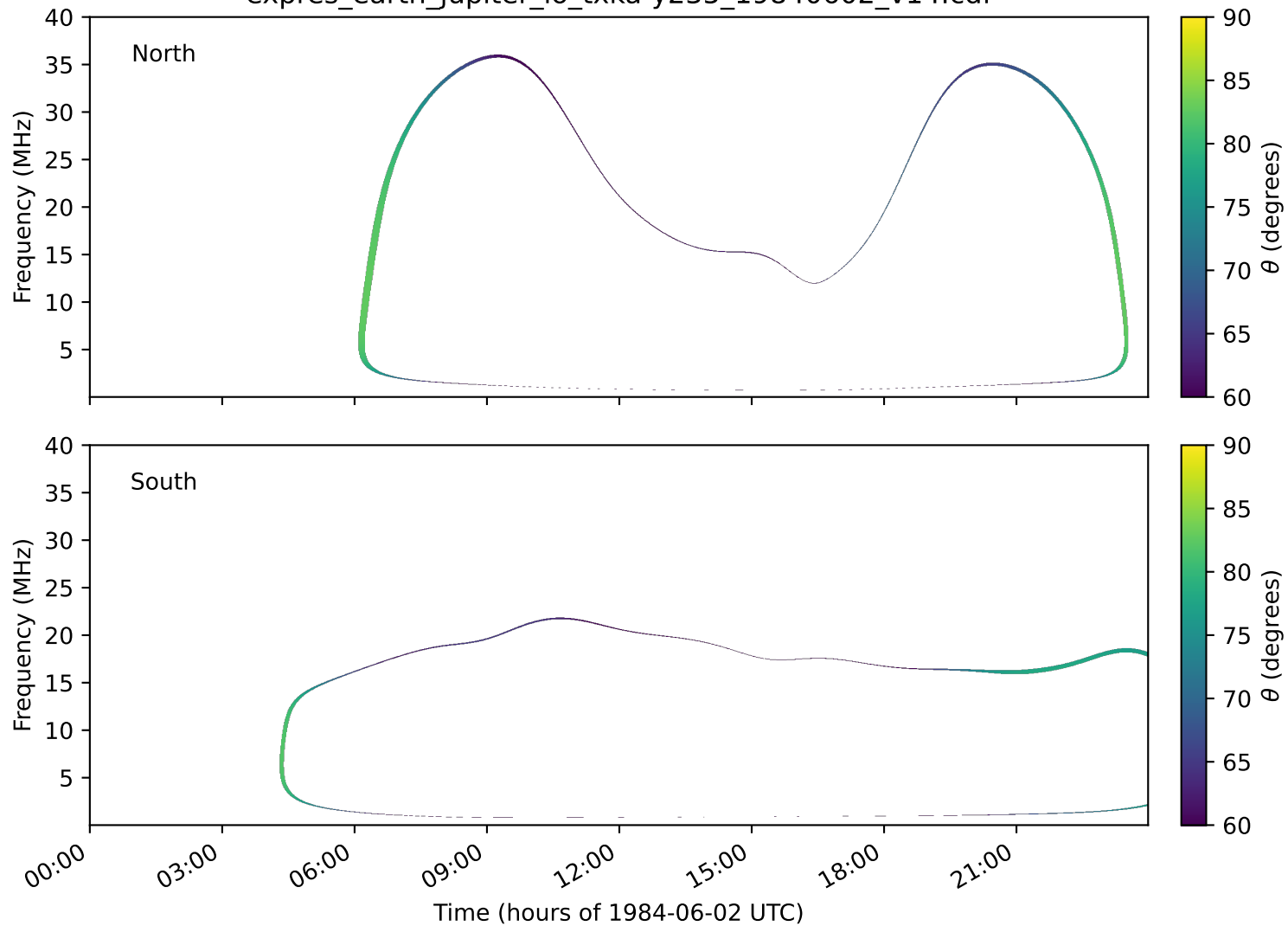
expres_earth_jupiter_io_txka-y235_19840602_v14.cdf
