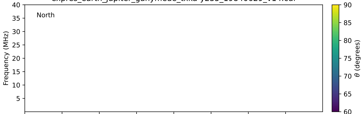
expres_earth_jupiter_ganymede_txka-y235_19840629_v14.cdf
