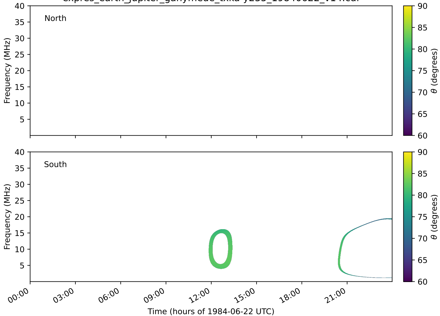
expres_earth_jupiter_ganymede_txka-y235_19840622_v14.cdf
