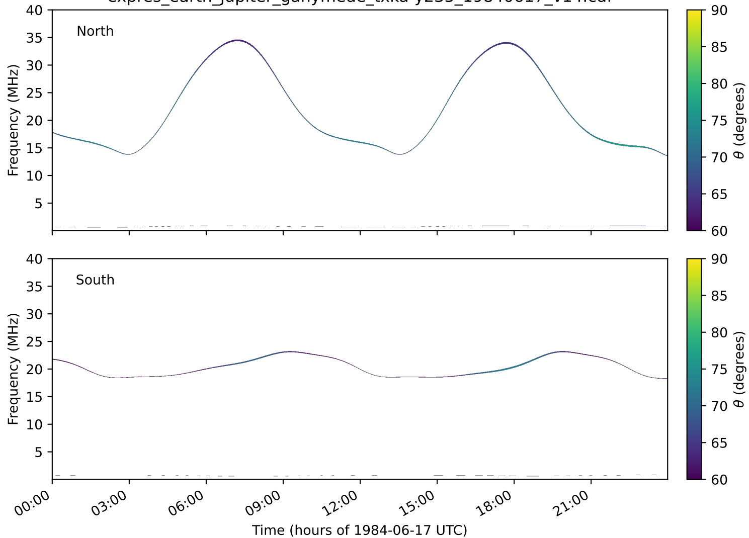
expres_earth_jupiter_ganymede_txka-y235_19840617_v14.cdf
