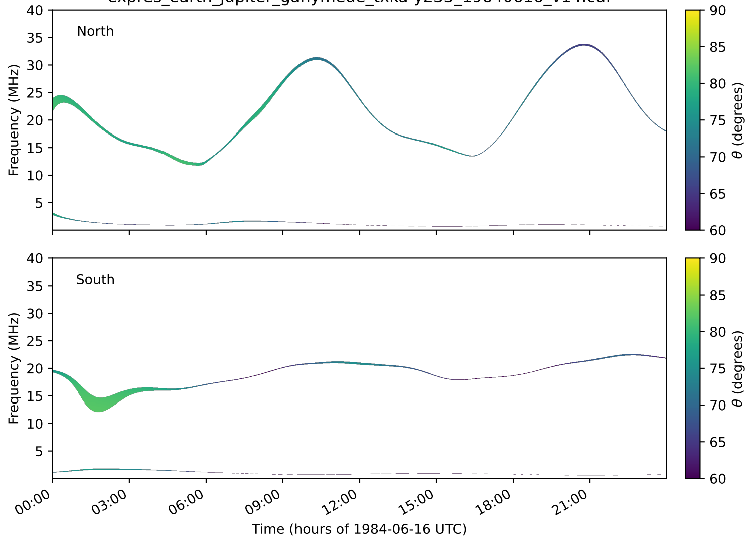
expres_earth_jupiter_ganymede_txka-y235_19840616_v14.cdf
