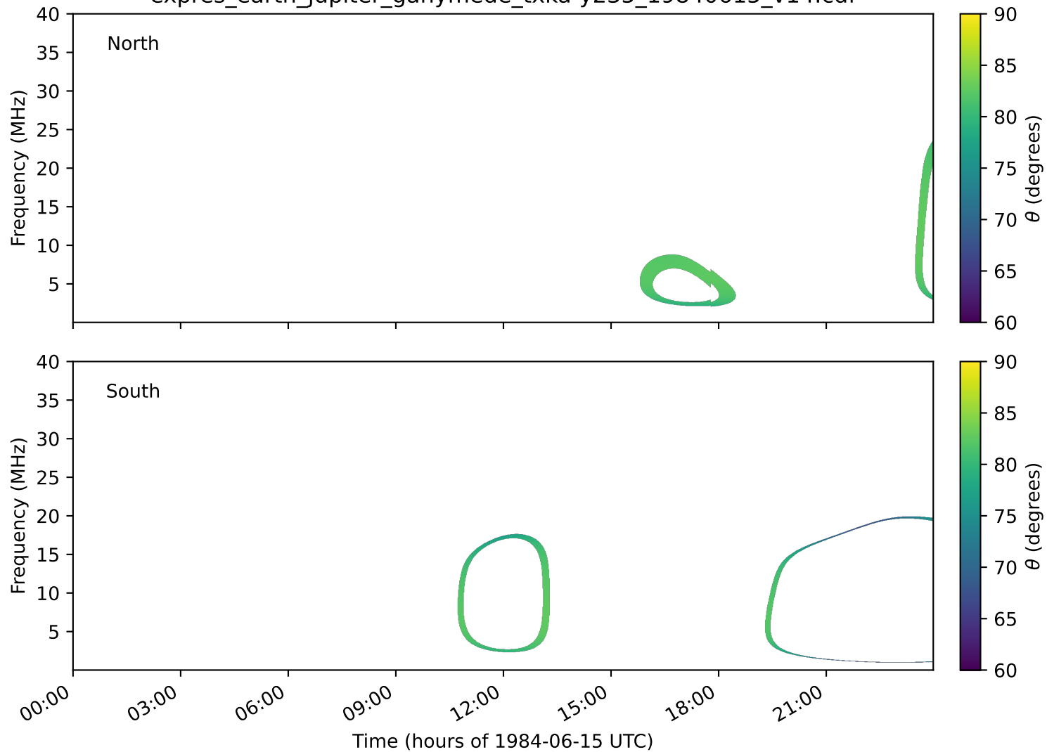
expres_earth_jupiter_ganymede_txka-y235_19840615_v14.cdf
