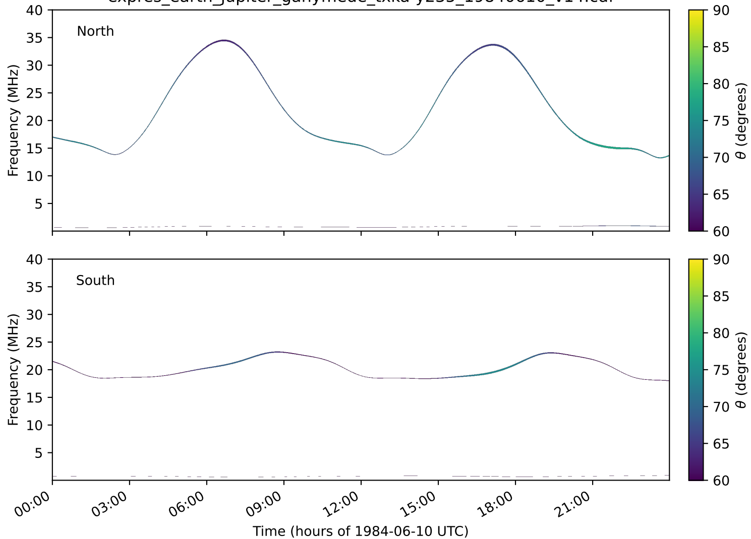
expres_earth_jupiter_ganymede_txka-y235_19840610_v14.cdf
