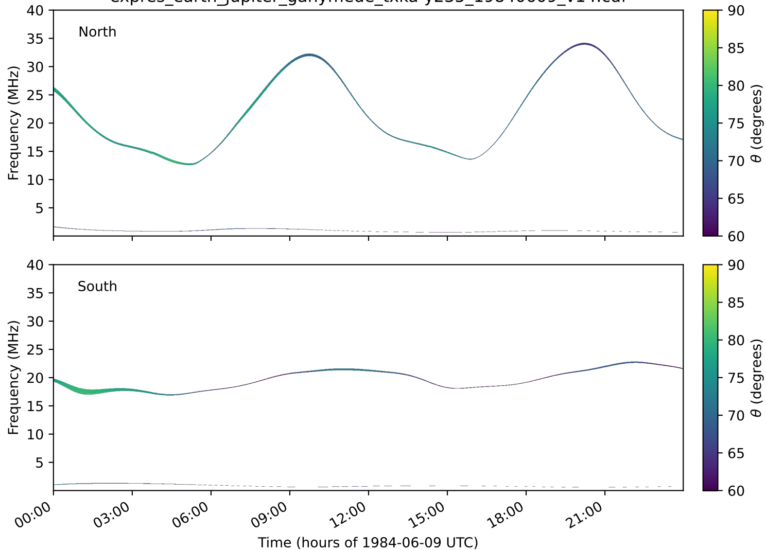
expres_earth_jupiter_ganymede_txka-y235_19840609_v14.cdf
