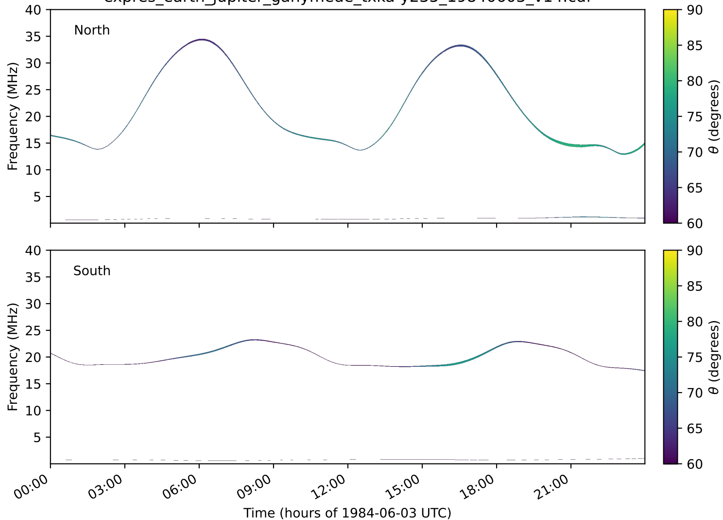
expres_earth_jupiter_ganymede_txka-y235_19840603_v14.cdf
