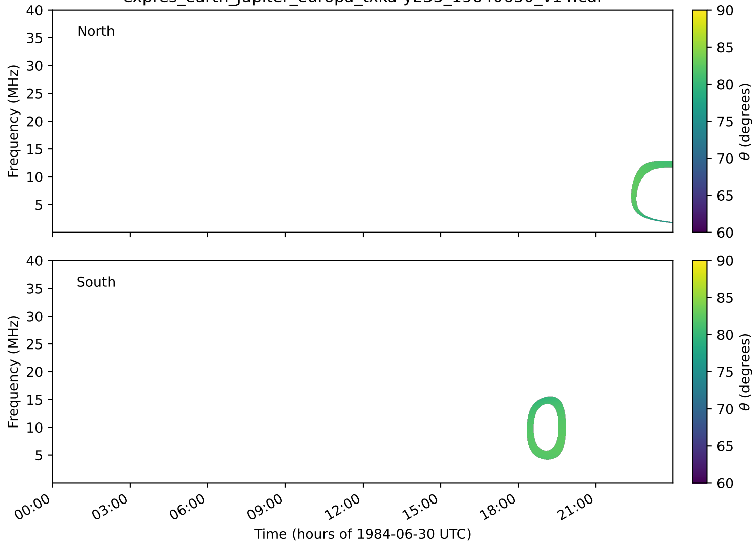
expres_earth_jupiter_europa_txka-y235_19840630_v14.cdf
