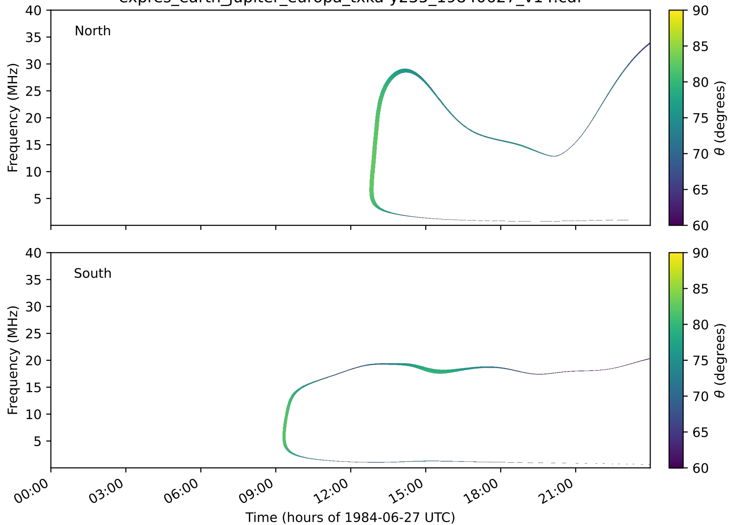
expres_earth_jupiter_europa_txka-y235_19840627_v14.cdf
