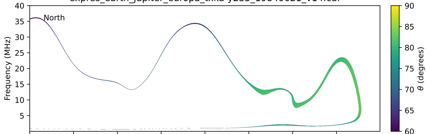
expres_earth_jupiter_europa_txka-y235_19840621_v14.cdf
