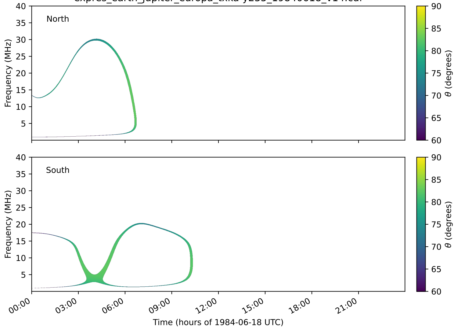
expres_earth_jupiter_europa_txka-y235_19840618_v14.cdf
