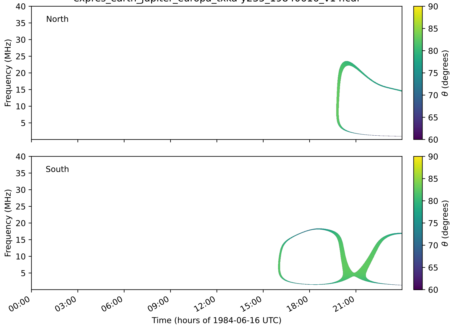
expres_earth_jupiter_europa_txka-y235_19840616_v14.cdf
