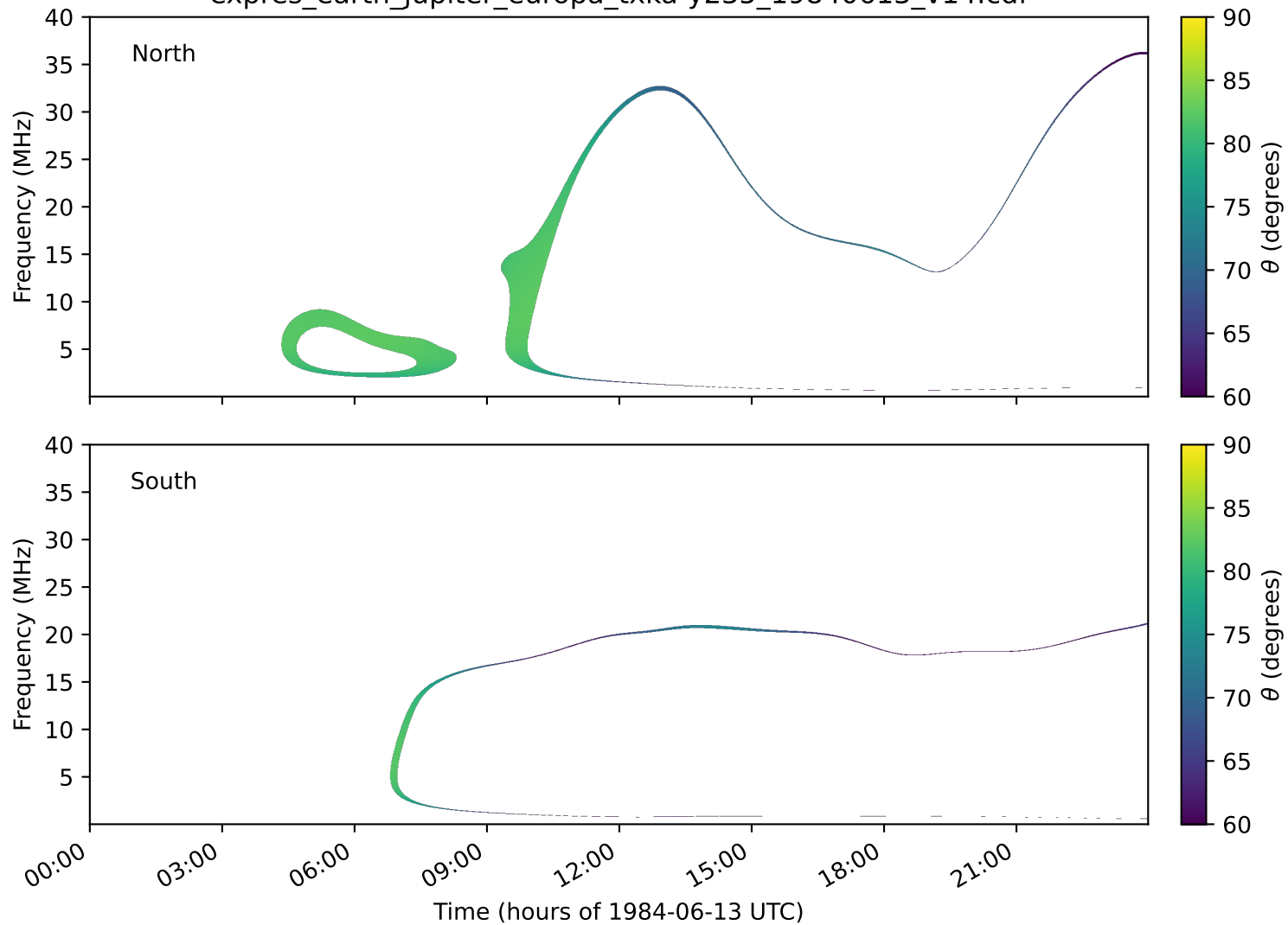
expres_earth_jupiter_europa_txka-y235_19840613_v14.cdf
