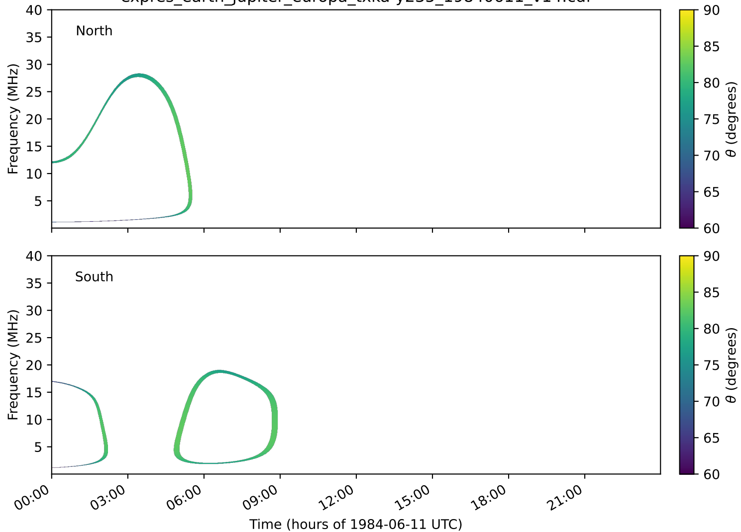
expres_earth_jupiter_europa_txka-y235_19840611_v14.cdf
