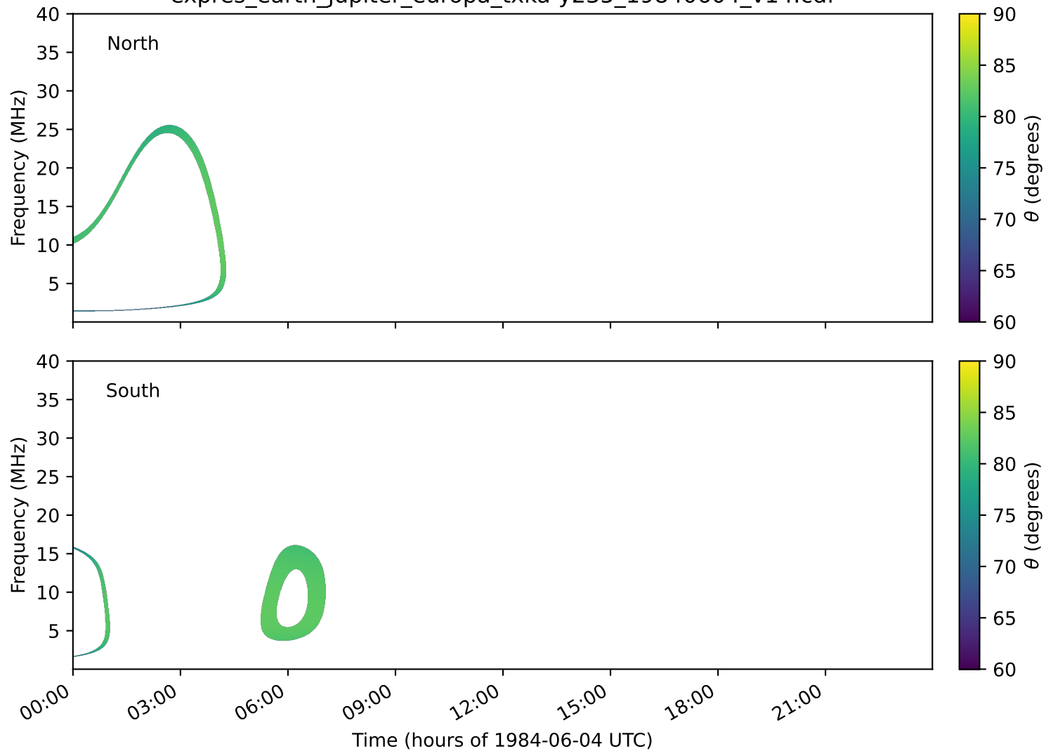
expres_earth_jupiter_europa_txka-y235_19840604_v14.cdf
